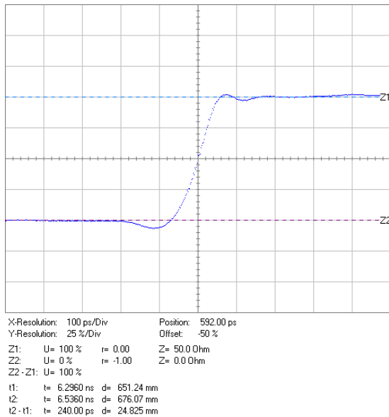
Example 1: Rising edge of a test generator pulse
