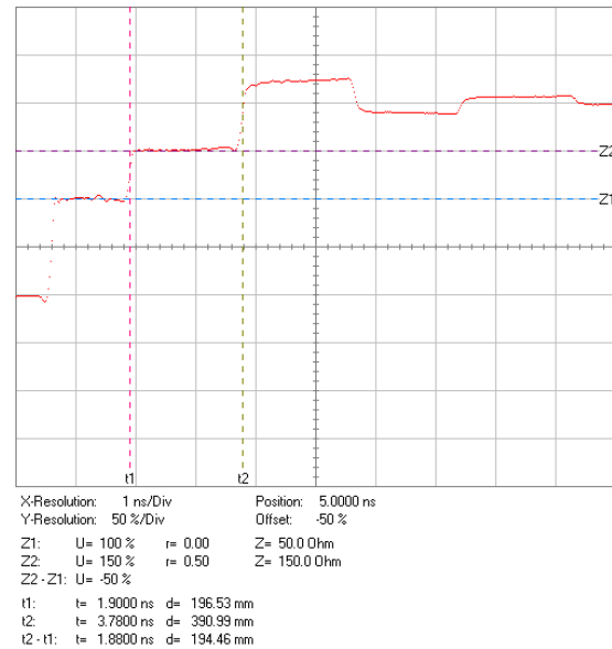
Example 2: Multiple reflections on an open 150 \Omega line
