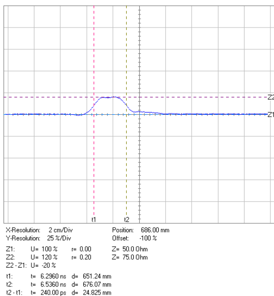
Example 3: Reflection of a 75 \Omega line inserted into a 50 \Omega line
