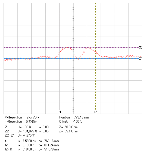
Example 4: BNC-connectors inserted into a 50 \Omega coax line (RG58)
